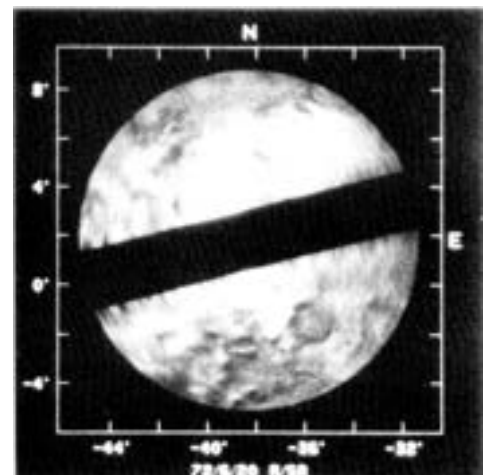
Close-up of an equatorial region on Venus as seen by radar astronomy from Earth. The diagonal bar is a region from which no useful data were returned. Several craters are seen, the largest almost 200 kilometers across. Craters on Venus are very shallow compared with crater of similar diameters on other worlds, hinting at some special erosion mechanism. Goldstone Tracking Station, Jet Propulsion Laboratory.
