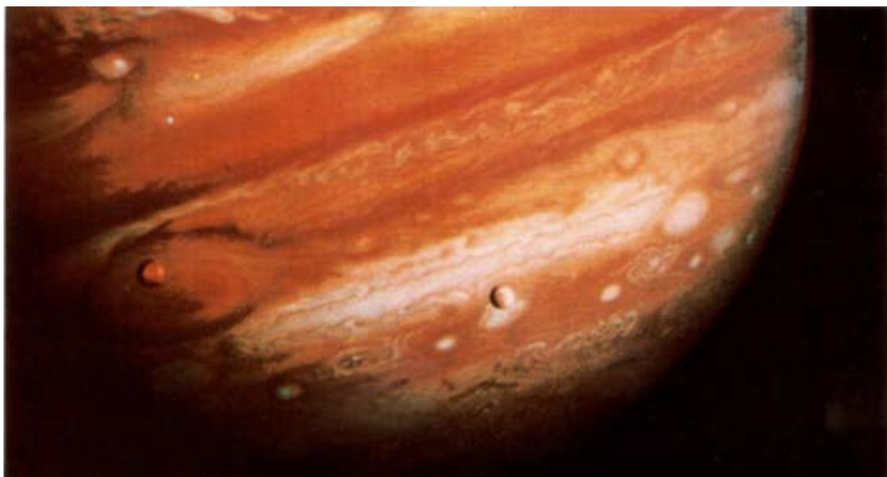
Voyager 1 far encounter image ( top ) of Jupiter from a range of 28 million kilometers. Bottom : Voyager approaches Jupiter with the moons Io and Callisto in foreground. Courtesy NASA.
