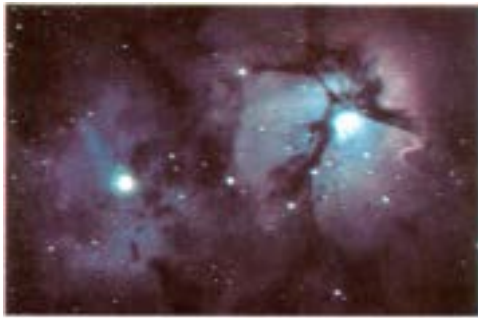
The Triffid Nebula in the constellation Sagittarius, several thousand light-years away. Stars embedded in the nebula induce the gas to shine. Most of the stars we see here are not associated with the nebula, but lie between it and us. The dark lanes in the nebula are composed of interstellar dust. Courtesy Hale Observatories.
