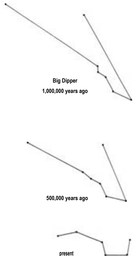
Computer-generated images of the Big Dipper as it would have been seen on Earth one million years ago and half a million years ago. Its present appearance is shown at bottom.
