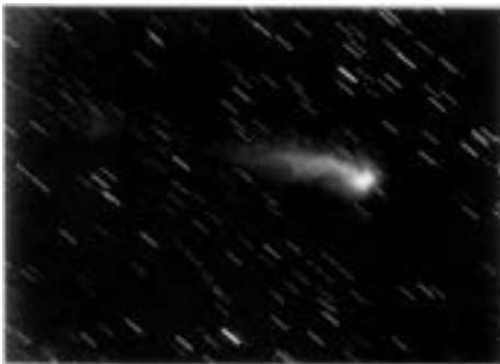
Comet Humason, photographed with the 48-inch Schmidt telescope of the Hale Observatories, 1961, and named after its discoverer, Milton Humason (Chapter 10). In this time exposure, the streaks are distant stars.
