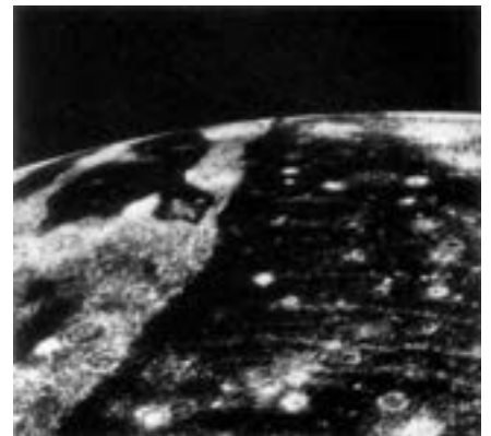
A Voyager 2 image of Ganymede on July 8, 1979. The parallel bright stripes extending across the dark plain at right might possibly have been caused, like ripples in a pond, by an ancient impact in this icy surface. There is no crater at the presumptive impact site, perhaps because of slow viscous deformation over the aeons. Courtesy NASA.
