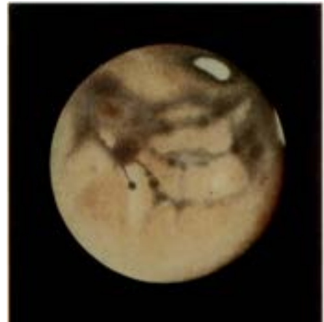
Drawing of Mars made in 1909 by E.M. Antoniadi in France. The polar cap and limb haze are apparent, but under excellent "seeing" conditions virtually no canals could be discerned.
