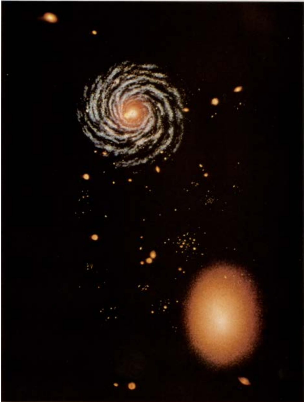
A small cluster of galaxies, including a spiral and an elliptical. Painting by Adolf Schaller.
