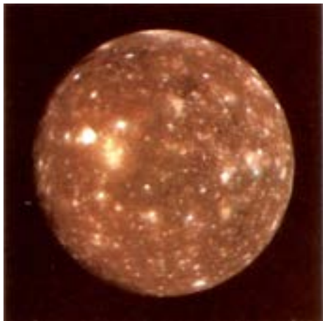
Callisto, the outermost large moon of Jupiter. Each circular bright spot is a large impact crater. Voyager 2 photo taken at a range of one million kilometers. Courtesy NASA.
