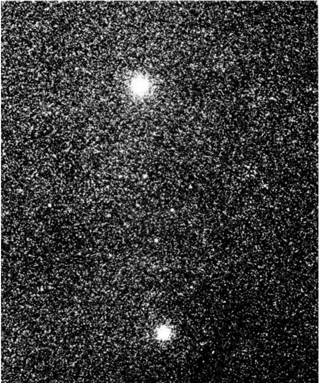
Globular star clusters gravitate about and demark the massive center of the Milky Way Galaxy. Many are located in a great spherical halo of stars and star clusters that encloses our spiral galaxy. A relative few, like these, are concentrated toward the galactic nucleus. From the planets of any one of these suns, the sky would be ablaze with stars. These globular clusters are designated NGC 6522 and NGC 6528, NGC being an abbreviation for “New General Catalog,” a compilation of clusters and galaxies. It was new when first compiled in 1888. Courtesy Kitt Peak National Observatory. © Association of Universities for Research in Astronomy, Inc., the Kitt Peak National Observatory.
