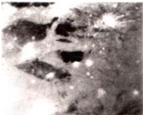
A region of Ganymede, largest moon of Jupiter. Bright ray craters and other impact scars are seen. Io and Europa, the other two large Jovian satellites, like the Earth, show few if any impact craters; erosion must be much more efficient there than on Ganymede and Callisto. Voyager 2 photo. Courtesy NASA.
