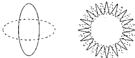
Figure 6.3 More frantic vibrational patterns have more energy than less frantic ones.
