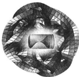
Figure 11.6 The world-sheet swept out by a string provides a shield that cancels the potentially cataclysmic effects associated with a tear in the fabric of space.
