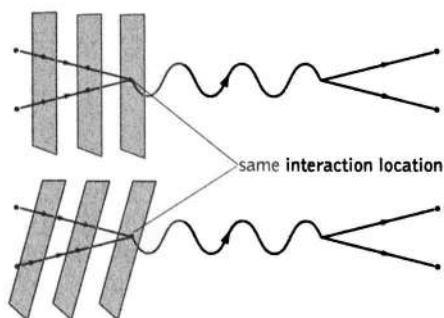
Figure 6.11 Observers in relative motion agree on when and where two point particles interact with another.
