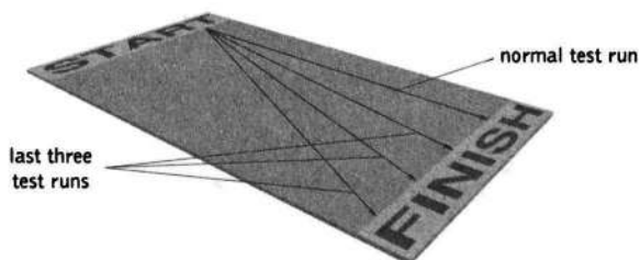
Figure 2.5 Due to the glaring late-afternoon sun, Slim drove at an increasingly greater angle on the last three runs.
