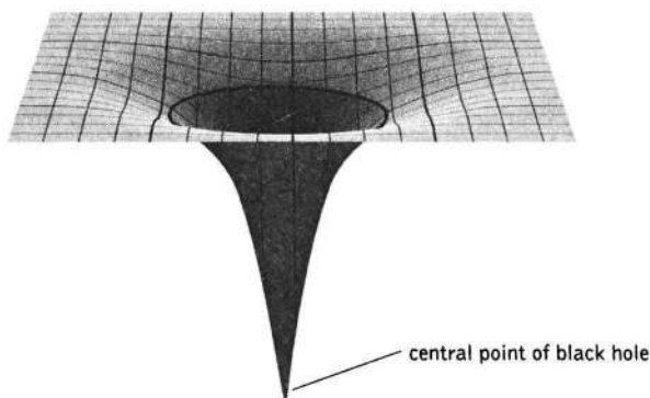
Figure 3.7 A black hole warps the surrounding spacetime fabric so severely that anything that comes within its “event horizon”—illustrated by the dark circle—can’t escape from its gravitational grip. No one knows exactly what happens at the deepest interior point of a black hole.
