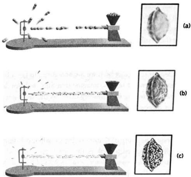
Figure 6.4 A peach pit is secured in a vise and it is drawn solely by observing how things—“probes”—thrown at it are deflected. By using ever smaller probes—(a) marbles, (b) five-millimeter pellets, (c) half-millimeter pellets—ever more detailed renditions can be drawn.
