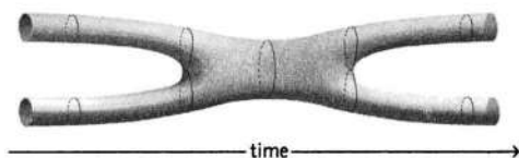
Figure 12.3 Strings interact by joining and splitting.
