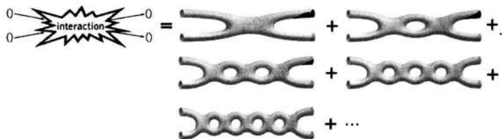
Figure 12.6 The net influence each incoming string has on the other comes from adding together the influences involving diagrams with ever more loops.
