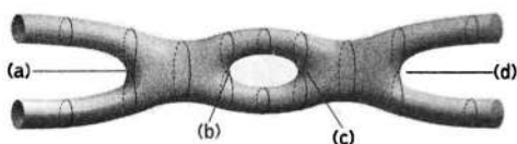
Figure 12.4 The quantum frenzy can cause a string/antistring pair to erupt (b) and annihilate (c), yielding a more complicated interaction.
