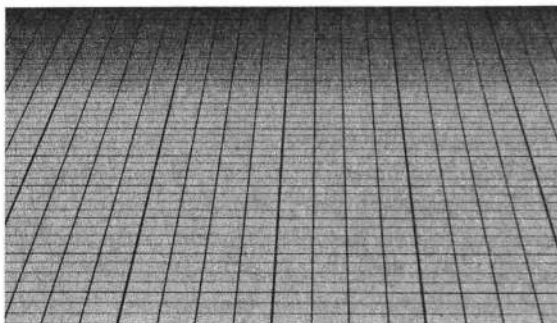
Figure 3.3 A schematic representation of flat space.
