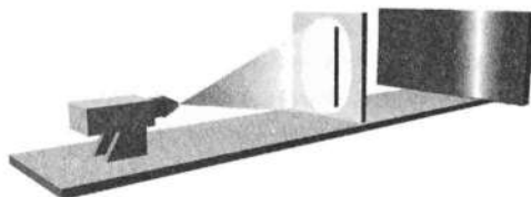
Figure 4.4 The right slit is open in this experiment, leading to an image on the photographic plate as shown.
