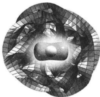
Figure 11.2 The highlighted region inside a Calabi-Yau shape contains a sphere.
