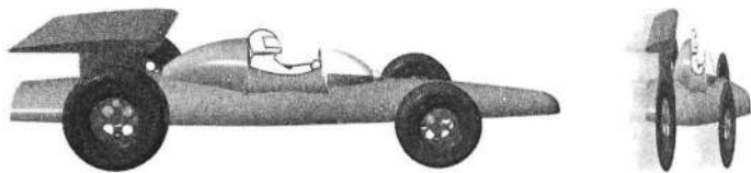
Figure 2.4 A moving object is shortened in the direction of its motion.
