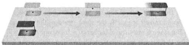
Figure 2.2 A stationary light clock in the foreground while a second light clock slides by at constant speed.
