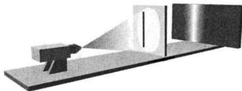
Figure 4.5 As in Figure 4.4, except now only the left slit is open.
