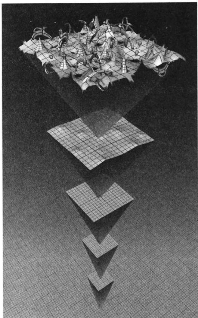
Figure 5.1 By sequentially magnifying a region of space, its ultramicroscopic properties can be probed. Attempts to merge general relativity and quantum mechanics run up against the violent quantum foam emerging at the highest level of magnification.
