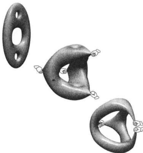
Figure 10.4 Orbifolding is a procedure in which a new Calabi-Yau shape is produced by gluing together various points on an initial Calabi-Yau shape.
