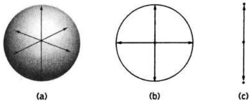
Figure 13.2 Spheres of dimensions that can be easily visualized—those of (a) two, (b) one, and (c) zero dimensions.
