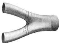
Figure 6.10 George and Gracie do not agree on the location of the interaction.
